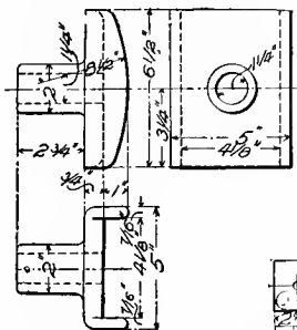
Figs. 1993-1995. Draw-bar Yoke-pocket Guide.
